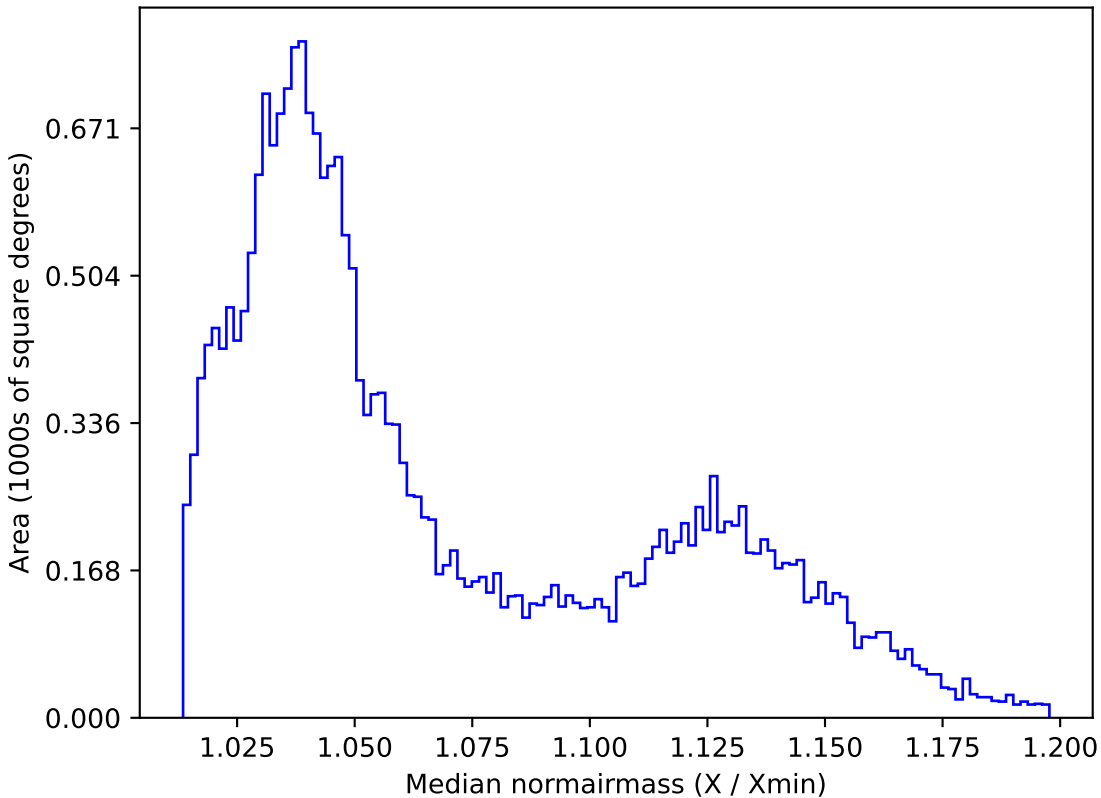
roll_pause_mjdp0_v3.4_10yrs All sky r band: Median normairmass
