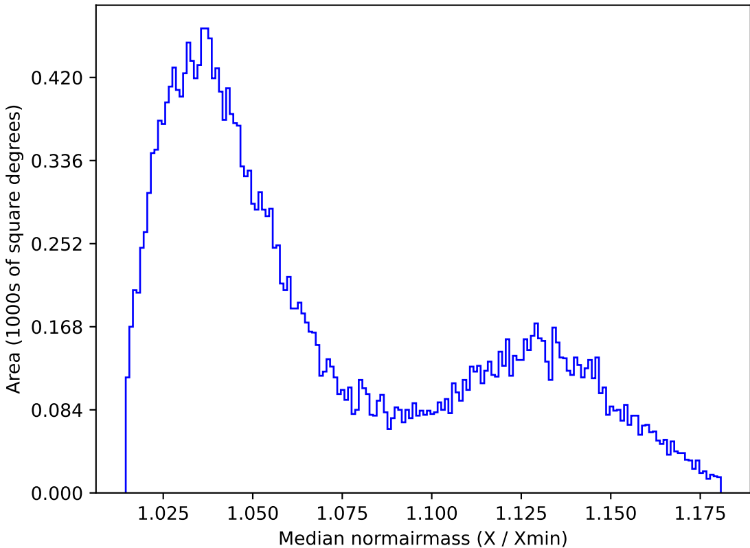
roll_pause_mjdp0_v3.4_10yrs All sky i band: Median normairmass
