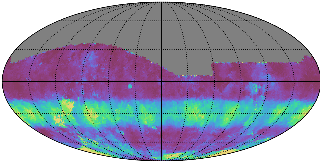
roll_pause_mjdp0_v3.4_10yrs All sky g band: Median normairmass
