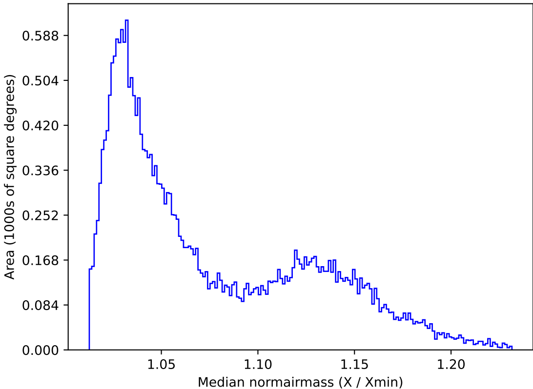
roll_pause_mjdp0_v3.4_10yrs All sky g band: Median normairmass
