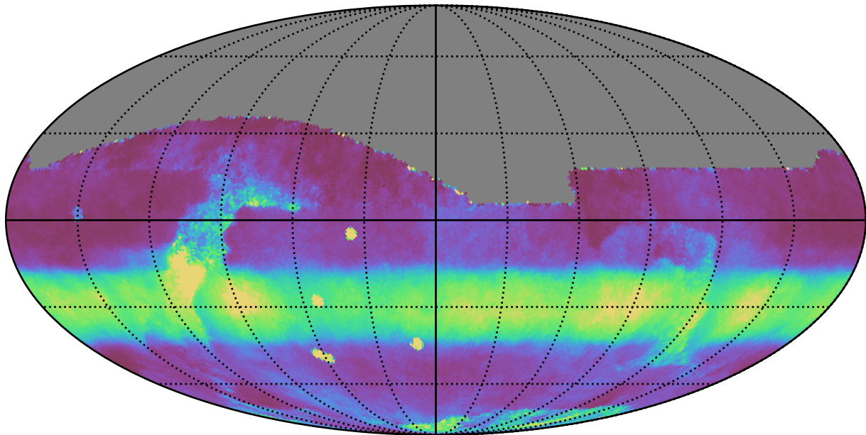
roll_pause_mjdp0_v3.4_10yrs All sky all bands: Median normairmass
