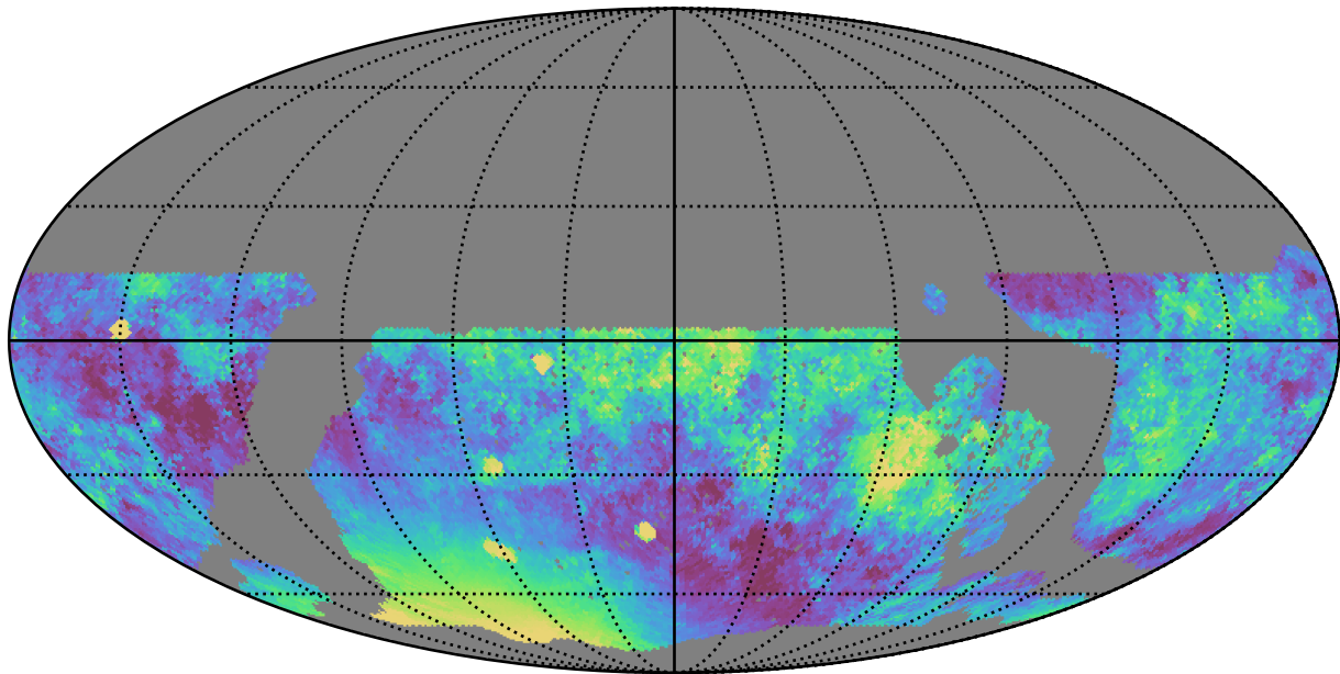
roll_pause_mjdp0_v3.4_10yrs WFD z band: Median moonDistance
