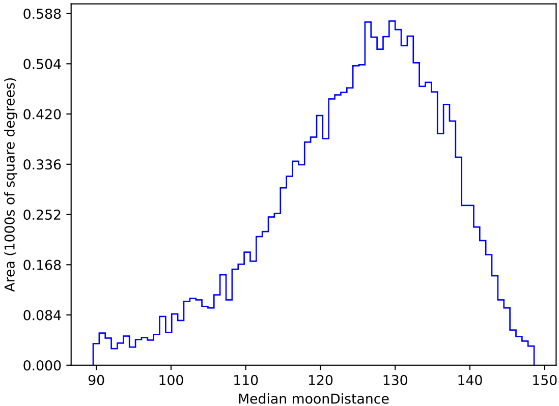
roll_pause_mjdp0_v3.4_10yrs WFD u band: Median moonDistance
