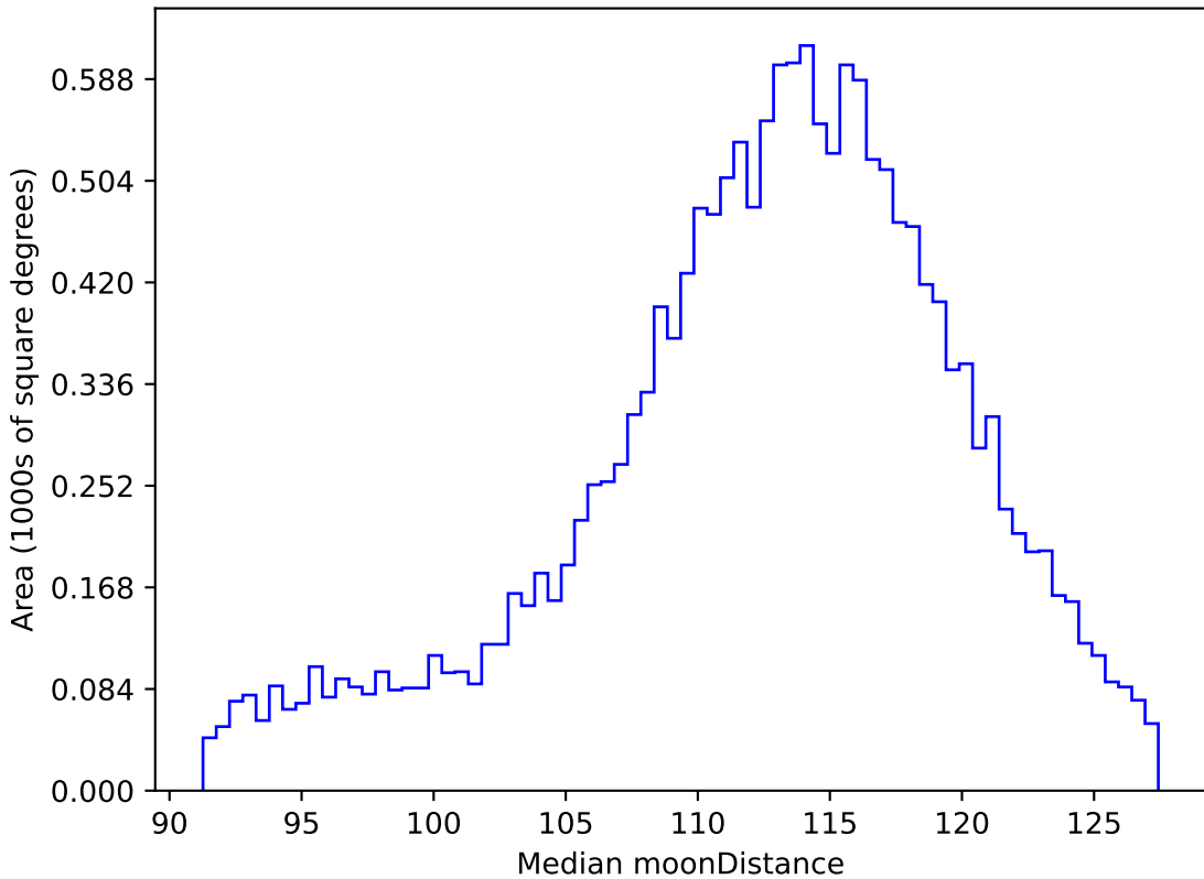
roll_pause_mjdp0_v3.4_10yrs WFD r band: Median moonDistance
