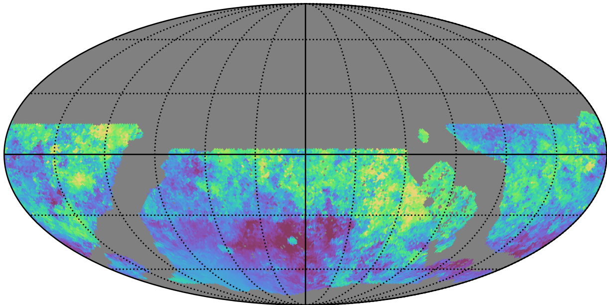
roll_pause_mjdp0_v3.4_10yrs WFD i band: Median moonDistance
