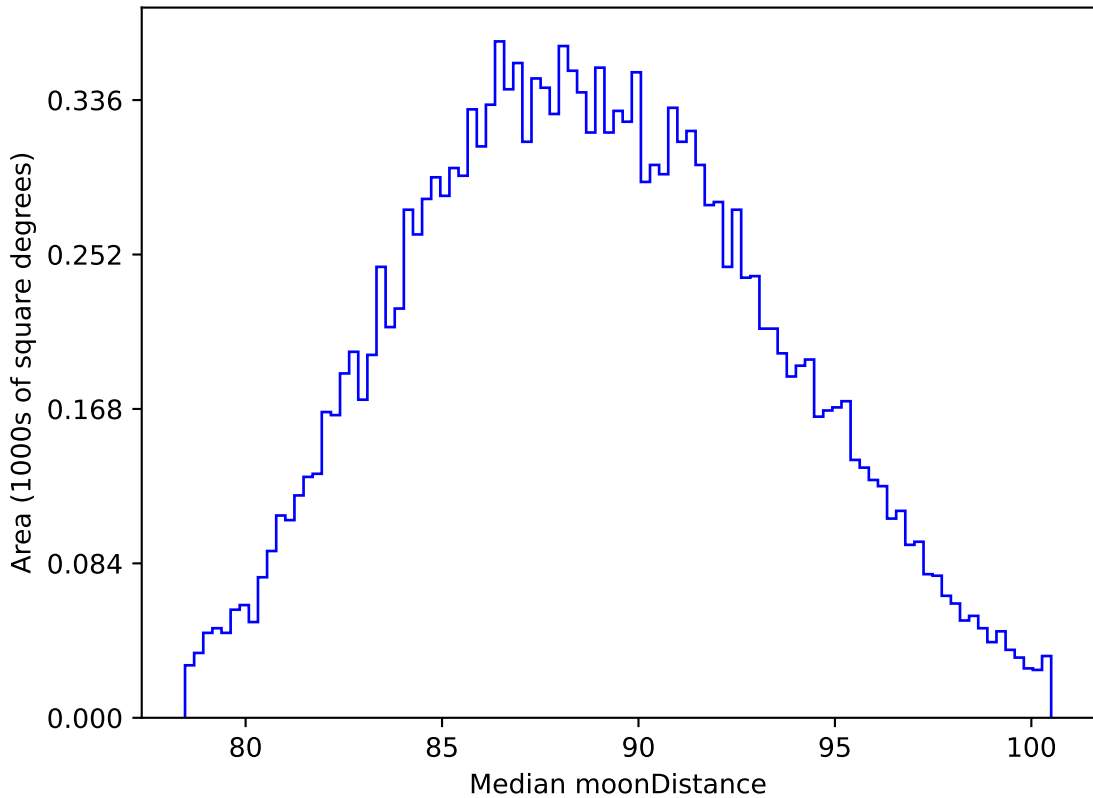
roll_pause_mjdp0_v3.4_10yrs WFD all bands: Median moonDistance
