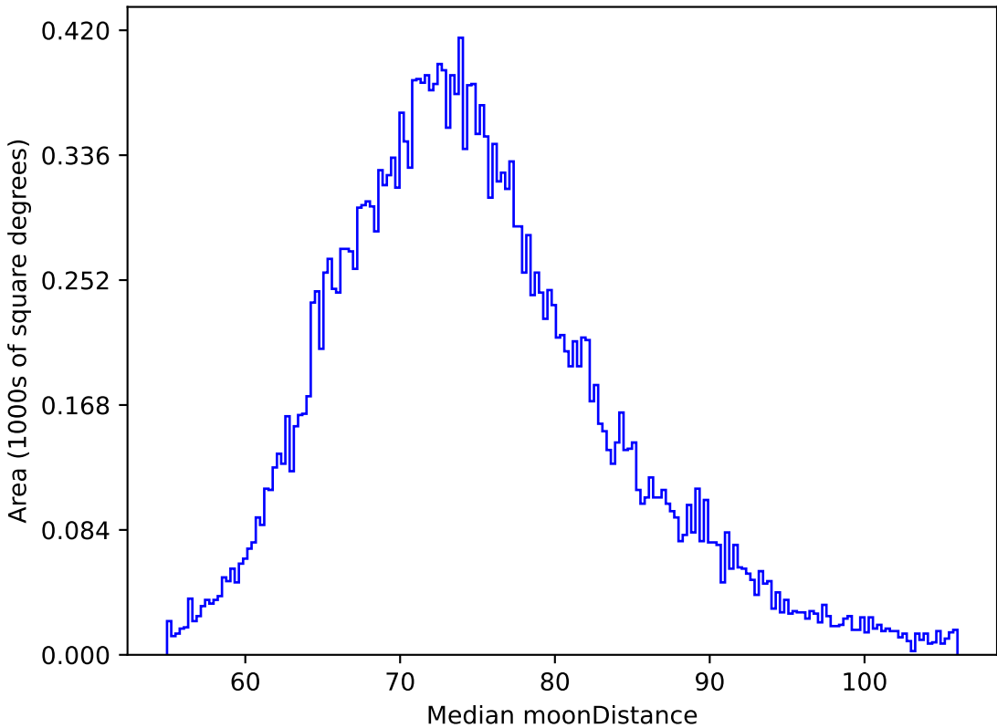
roll_pause_mjdp0_v3.4_10yrs All sky z band: Median moonDistance
