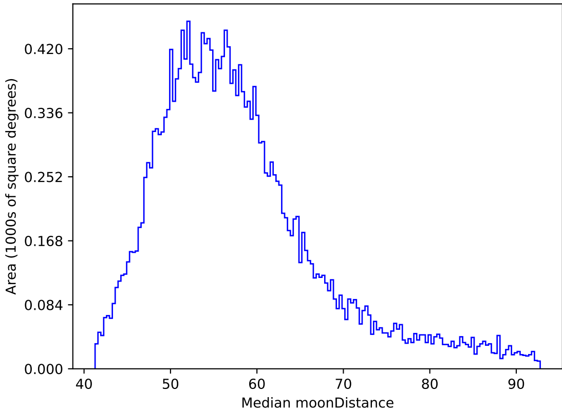
roll_pause_mjdp0_v3.4_10yrs All sky y band: Median moonDistance
