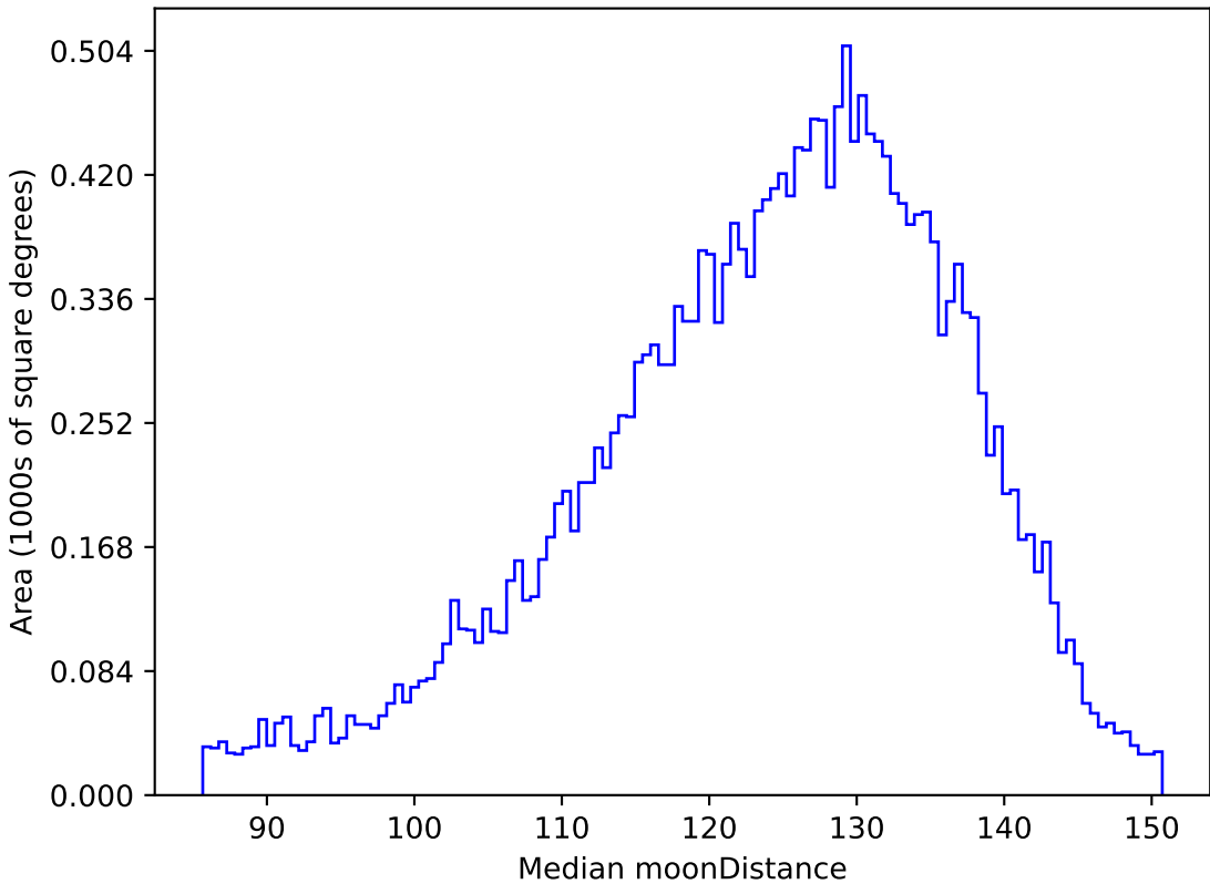
roll_pause_mjdp0_v3.4_10yrs All sky u band: Median moonDistance
