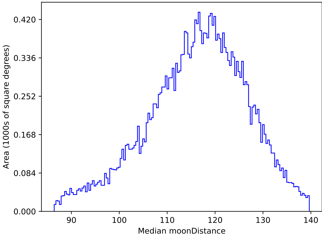
roll_pause_mjdp0_v3.4_10yrs All sky g band: Median moonDistance
