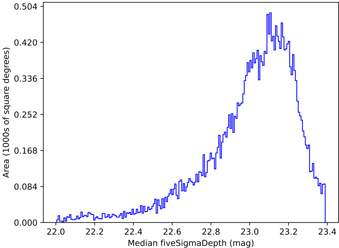
roll_pause_mjdp0_v3.4_10yrs Yr 1 z band: Median fiveSigmaDepth
