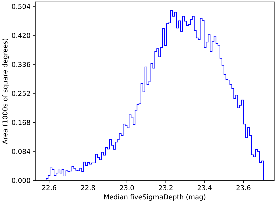
roll_pause_mjdp0_v3.4_10yrs Yr 1 u band: Median fiveSigmaDepth
