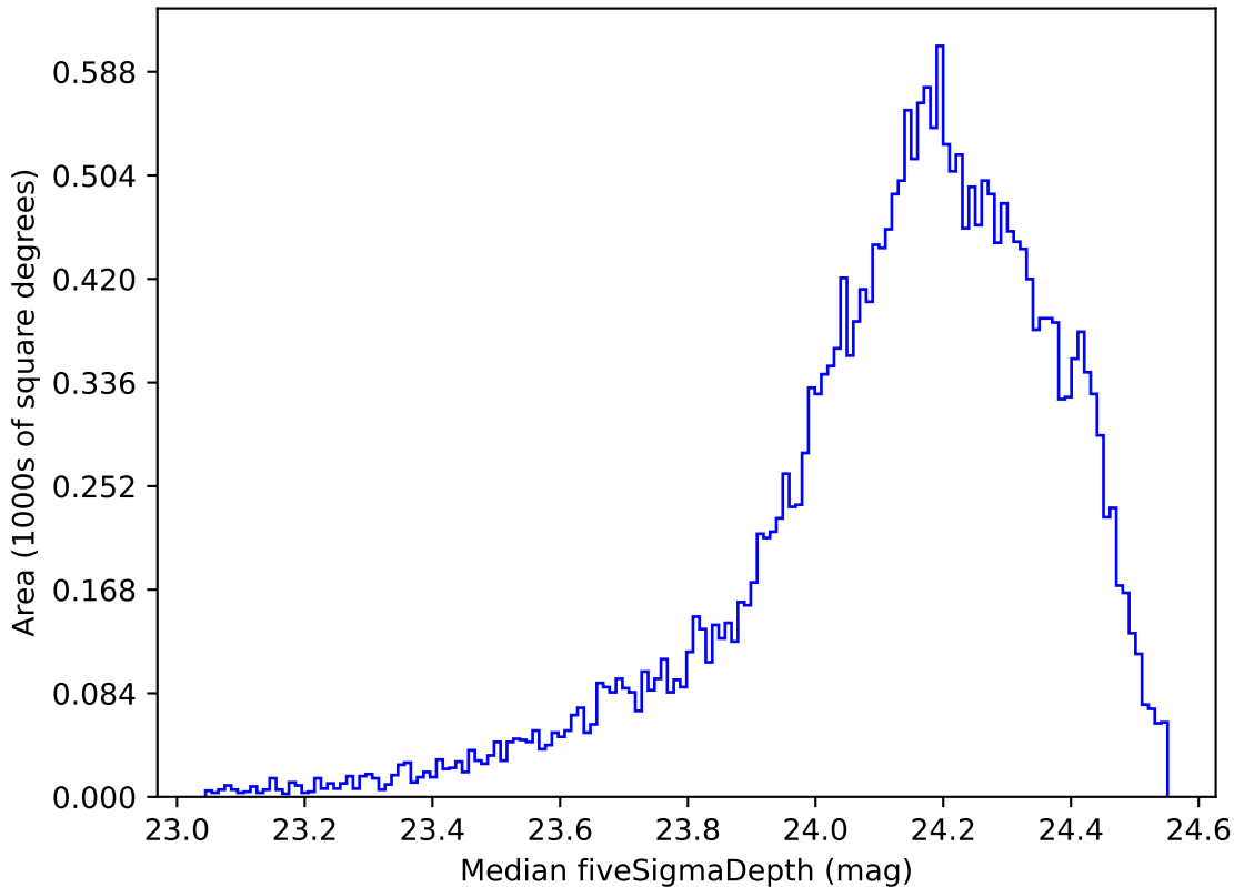
roll_pause_mjdp0_v3.4_10yrs Yr 1 r band: Median fiveSigmaDepth
