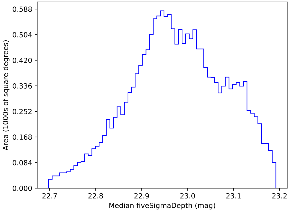
roll_pause_mjdp0_v3.4_10yrs WFD z band: Median fiveSigmaDepth
