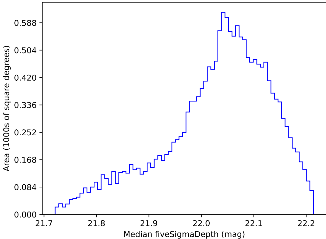
roll_pause_mjdp0_v3.4_10yrs WFD y band: Median fiveSigmaDepth
