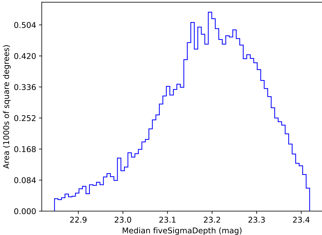
roll_pause_mjdp0_v3.4_10yrs WFD u band: Median fiveSigmaDepth
