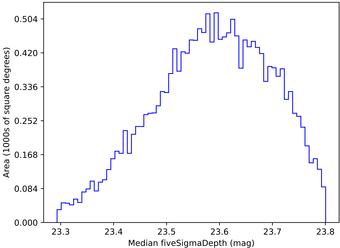
roll_pause_mjdp0_v3.4_10yrs WFD i band: Median fiveSigmaDepth
