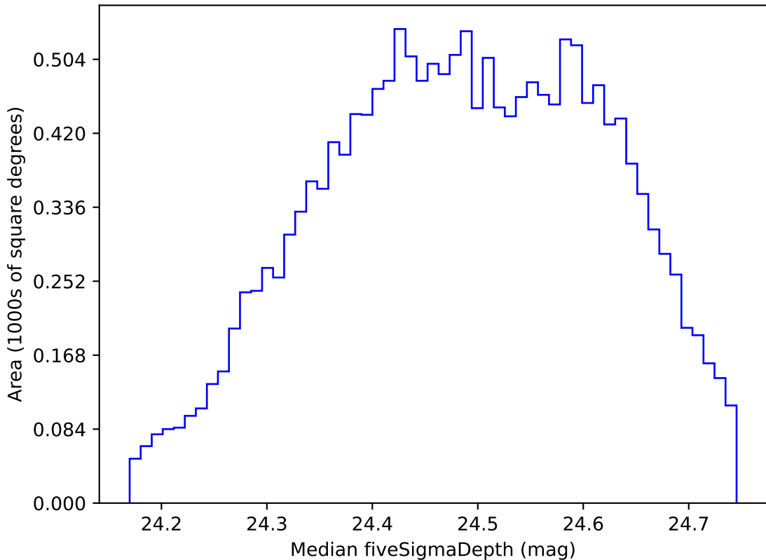
roll_pause_mjdp0_v3.4_10yrs WFD g band: Median fiveSigmaDepth
