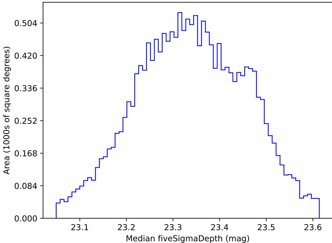
roll_pause_mjdp0_v3.4_10yrs WFD all bands: Median fiveSigmaDepth
