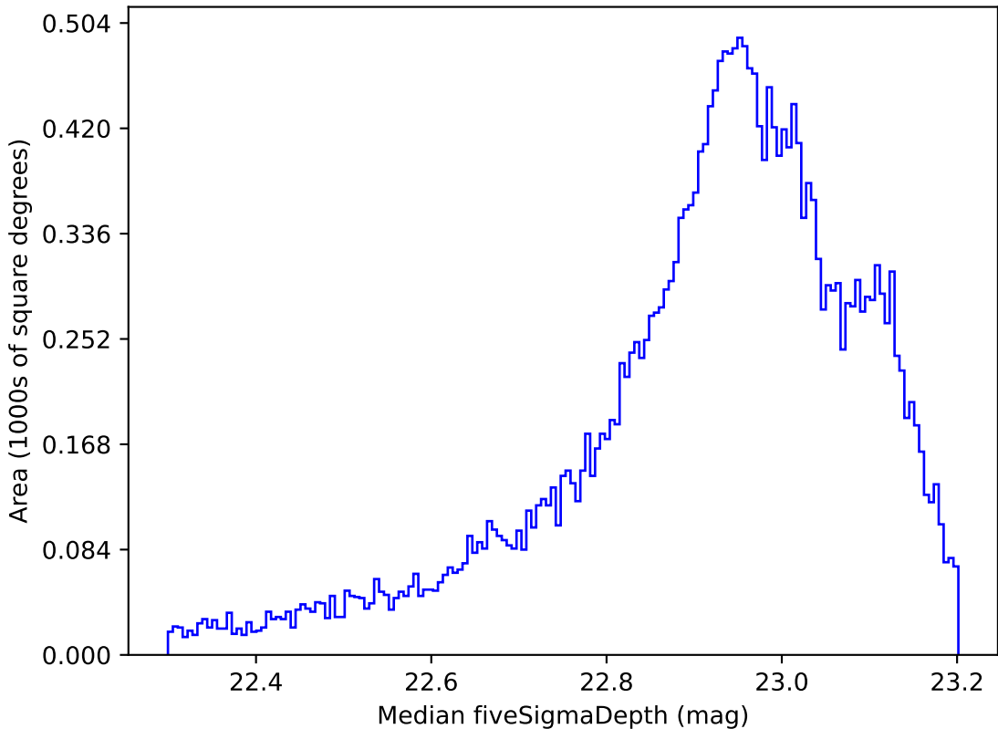
roll_pause_mjdp0_v3.4_10yrs All sky z band: Median fiveSigmaDepth
