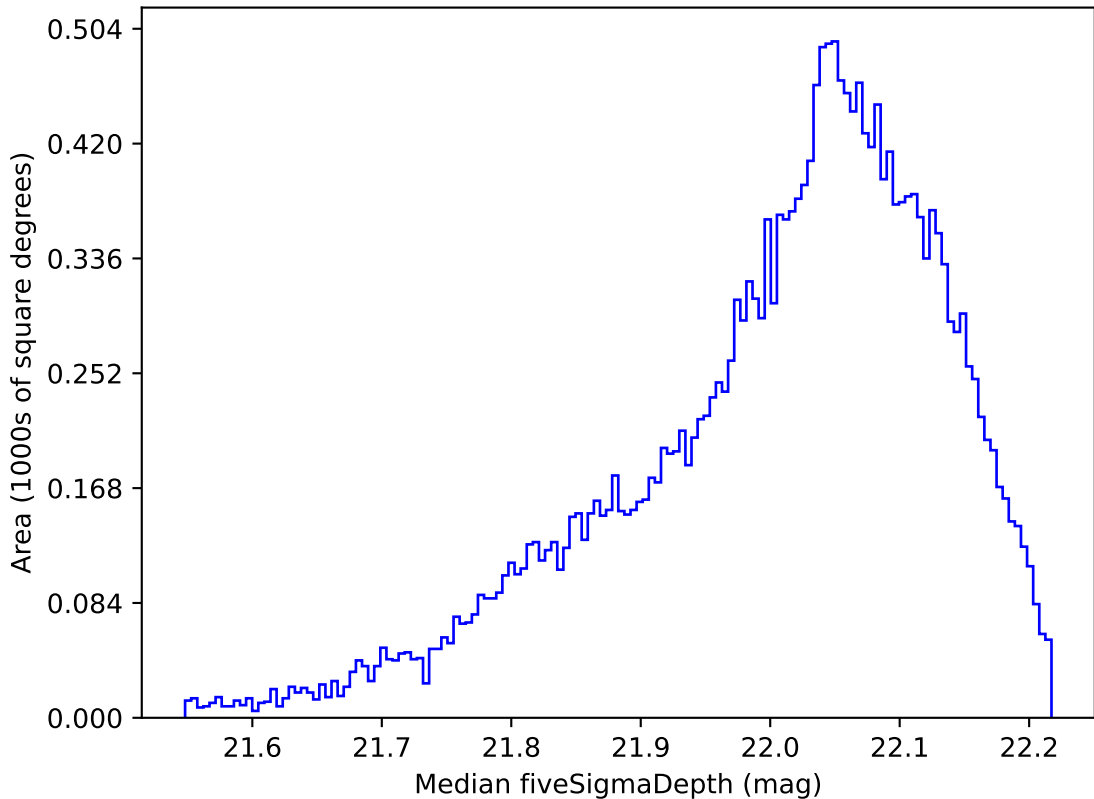
roll_pause_mjdp0_v3.4_10yrs All sky y band: Median fiveSigmaDepth
