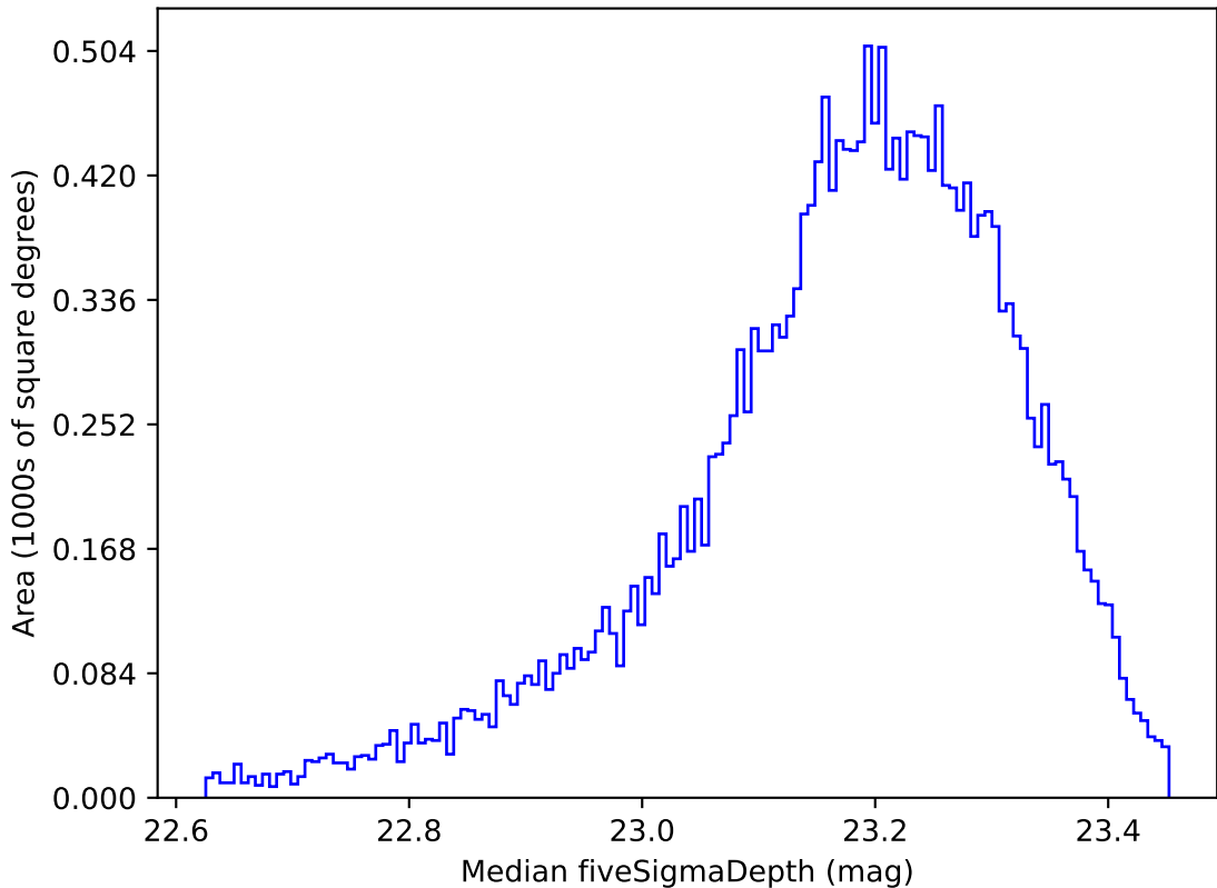
roll_pause_mjdp0_v3.4_10yrs All sky u band: Median fiveSigmaDepth
