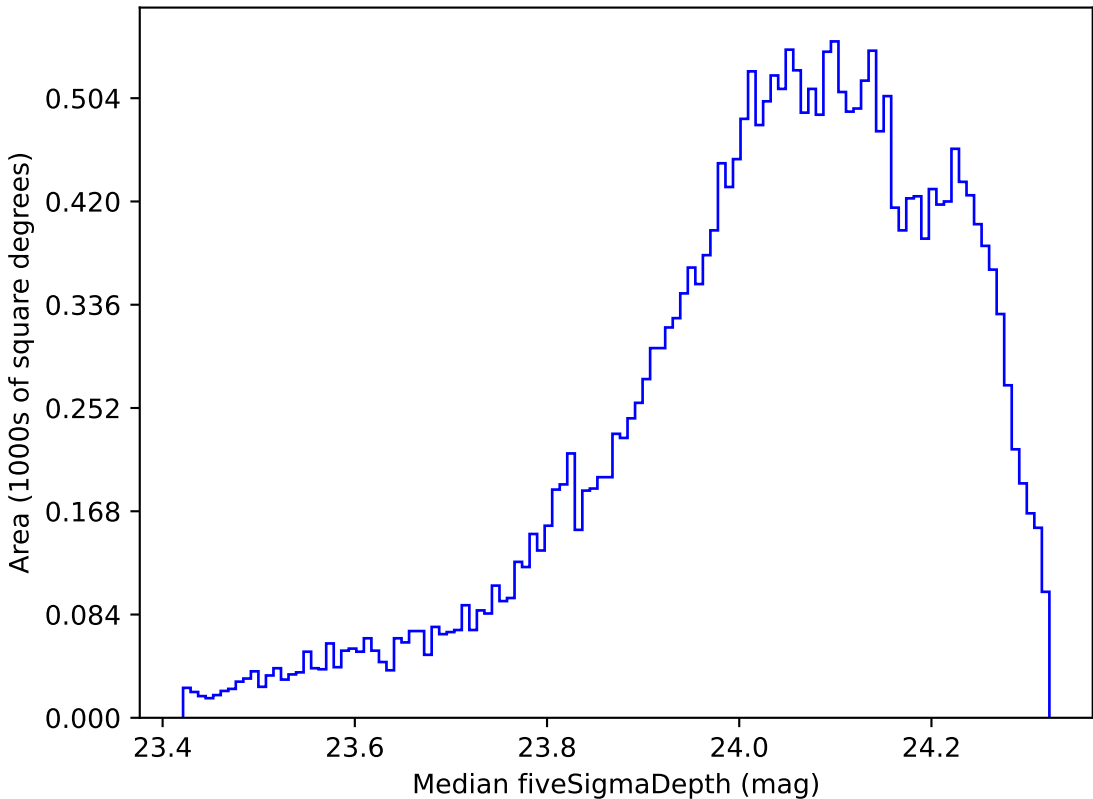
roll_pause_mjdp0_v3.4_10yrs All sky r band: Median fiveSigmaDepth
