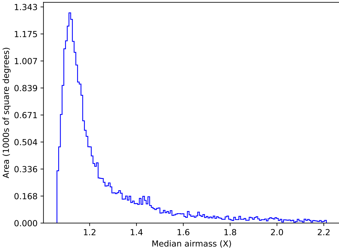
roll_pause_mjdp0_v3.4_10yrs Yr 1 z band: Median airmass
