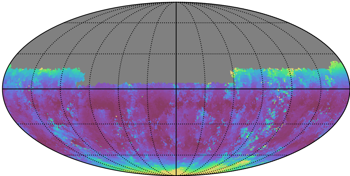
roll_pause_mjdp0_v3.4_10yrs Yr 1 u band: Median airmass
