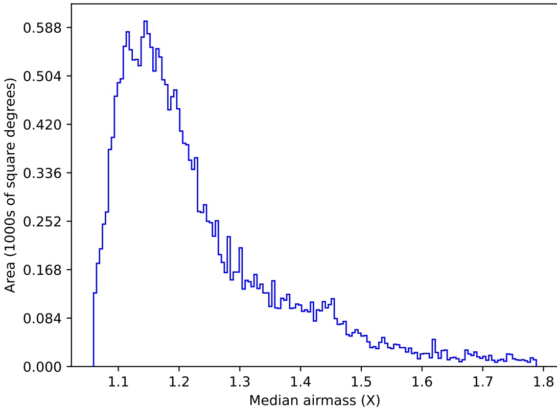
roll_pause_mjdp0_v3.4_10yrs Yr 1 u band: Median airmass
