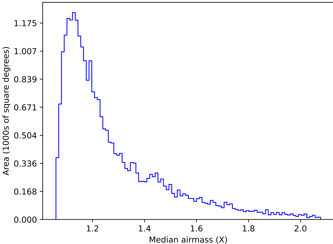
roll_pause_mjdp0_v3.4_10yrs Yr 1 g band: Median airmass
