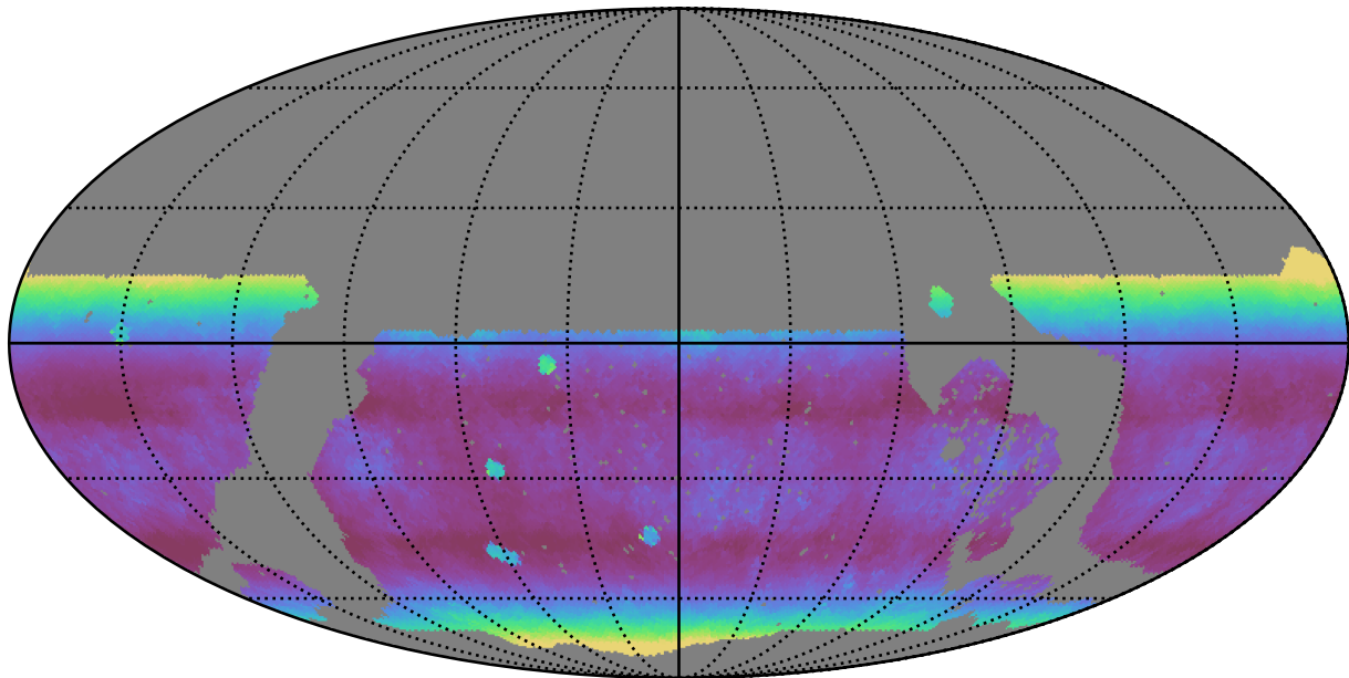
roll_pause_mjdp0_v3.4_10yrs WFD z band: Median airmass
