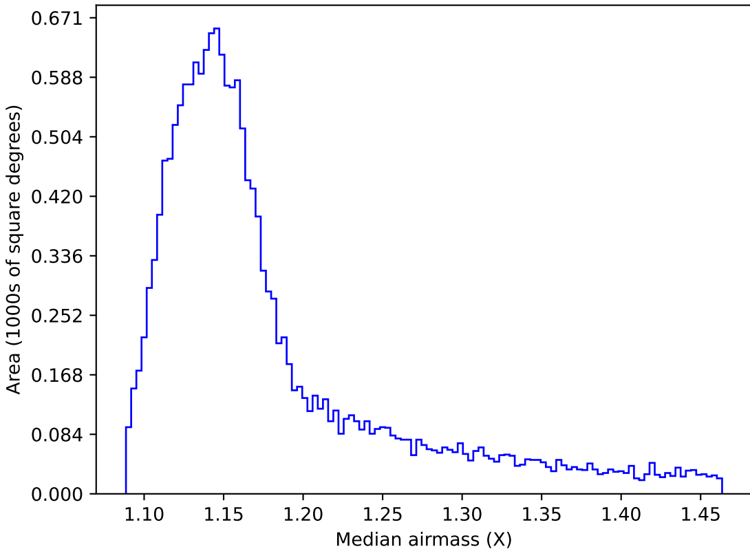
roll_pause_mjdp0_v3.4_10yrs WFD z band: Median airmass
