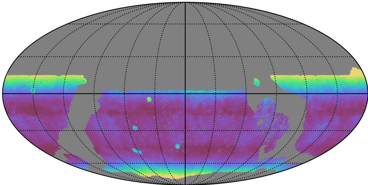
roll_pause_mjdp0_v3.4_10yrs WFD y band: Median airmass
