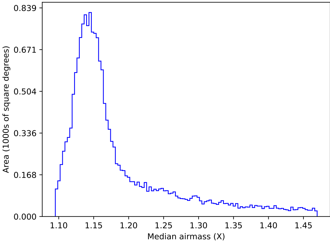
roll_pause_mjdp0_v3.4_10yrs WFD y band: Median airmass
