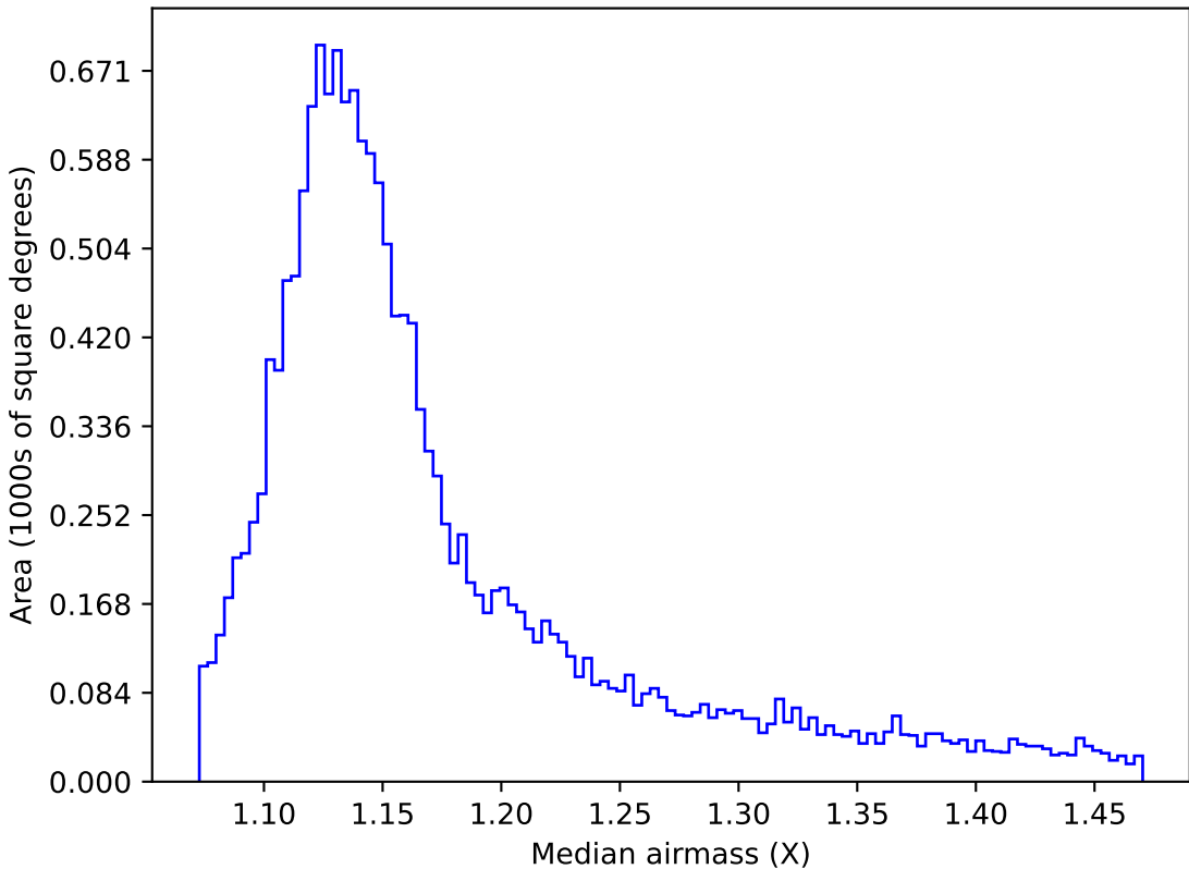
roll_pause_mjdp0_v3.4_10yrs WFD u band: Median airmass
