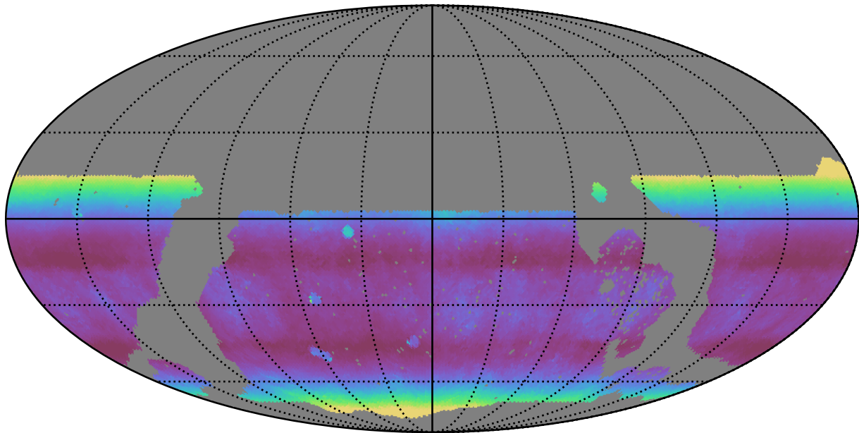
roll_pause_mjdp0_v3.4_10yrs WFD i band: Median airmass
