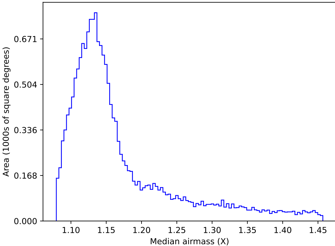
roll_pause_mjdp0_v3.4_10yrs WFD i band: Median airmass
