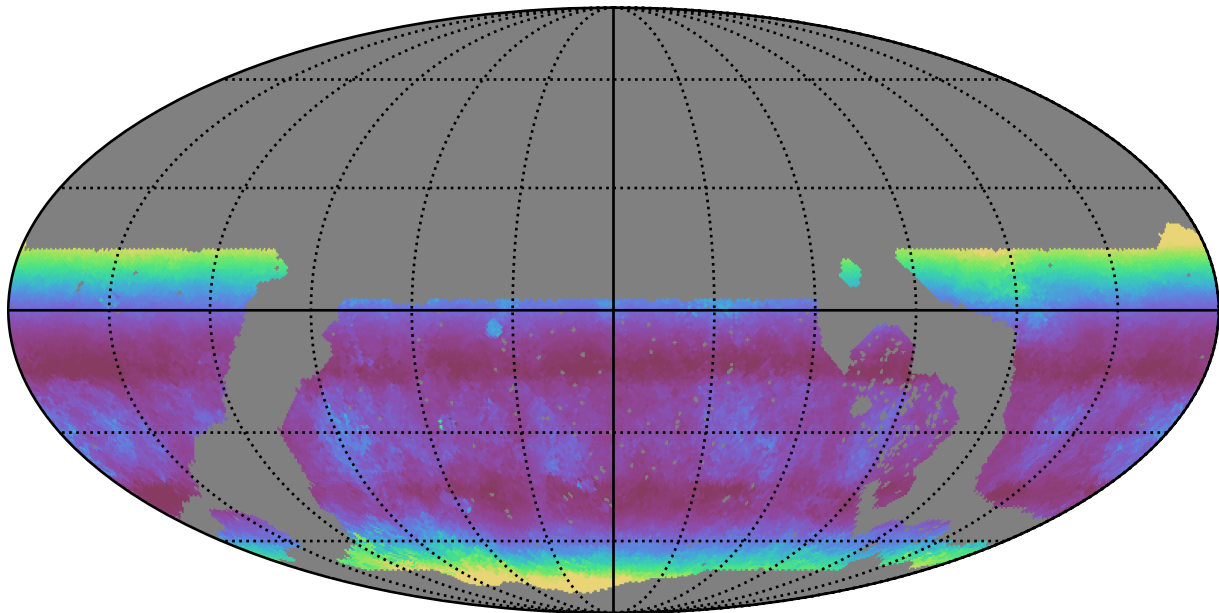
roll_pause_mjdp0_v3.4_10yrs WFD g band: Median airmass
