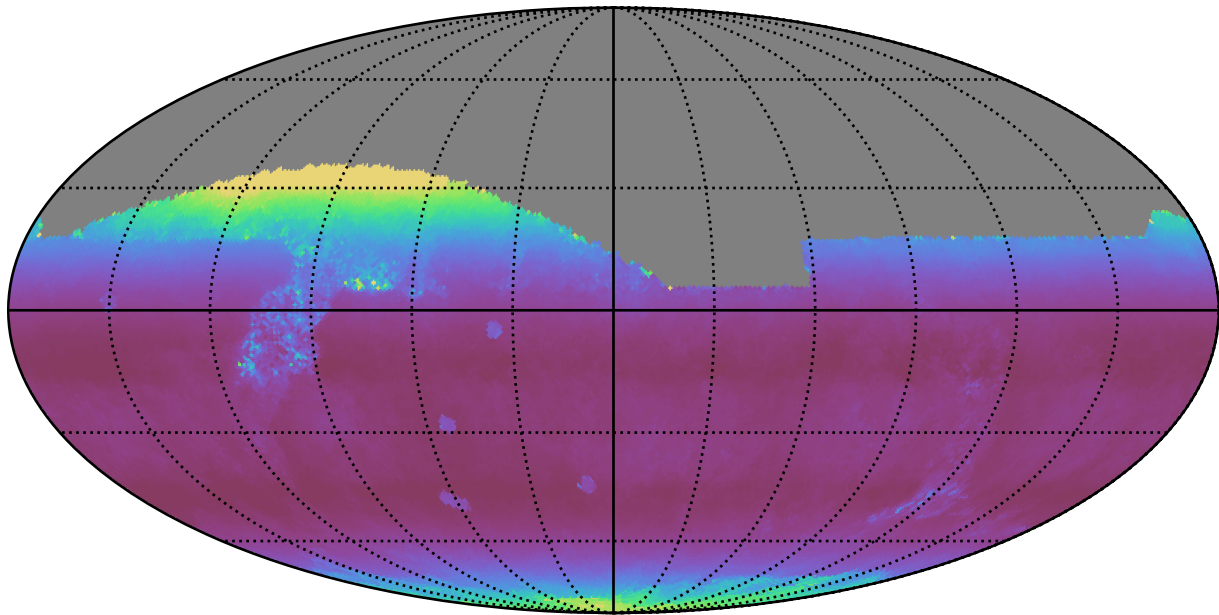
roll_pause_mjdp0_v3.4_10yrs All sky z band: Median airmass
