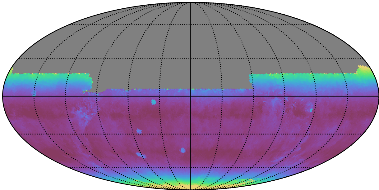
roll_pause_mjdp0_v3.4_10yrs All sky y band: Median airmass
