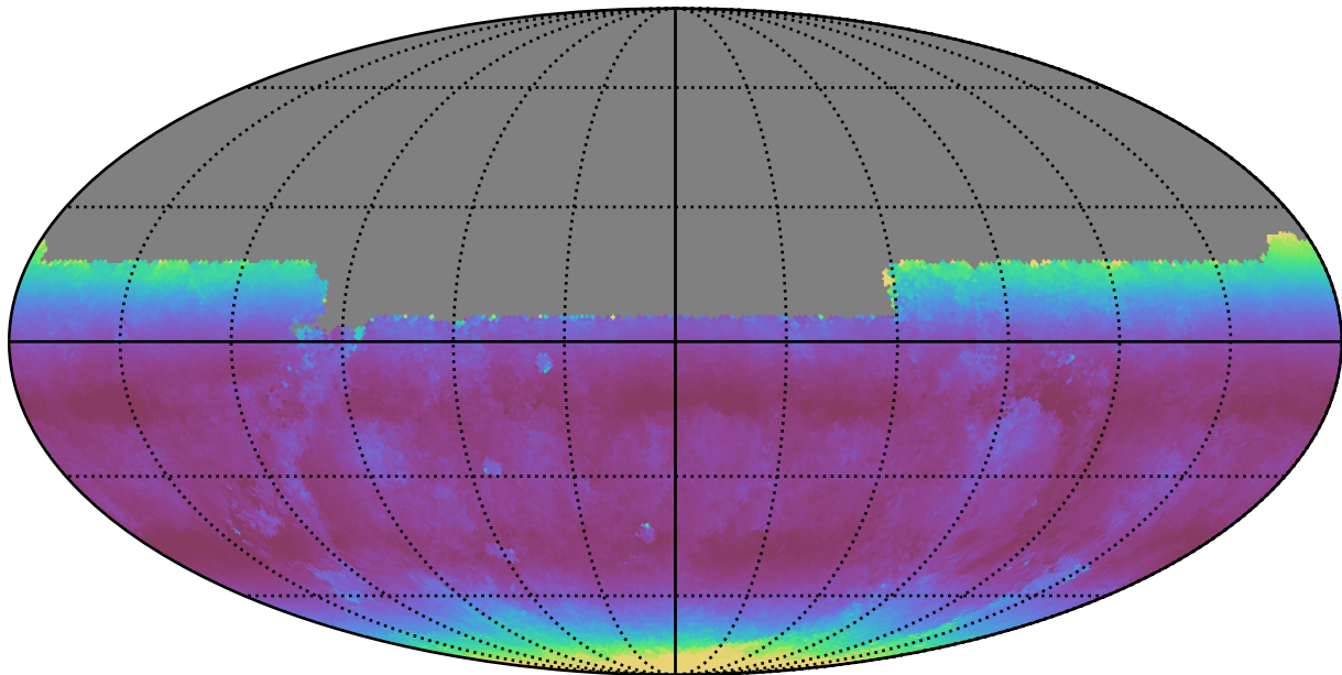
roll_pause_mjdp0_v3.4_10yrs All sky u band: Median airmass
