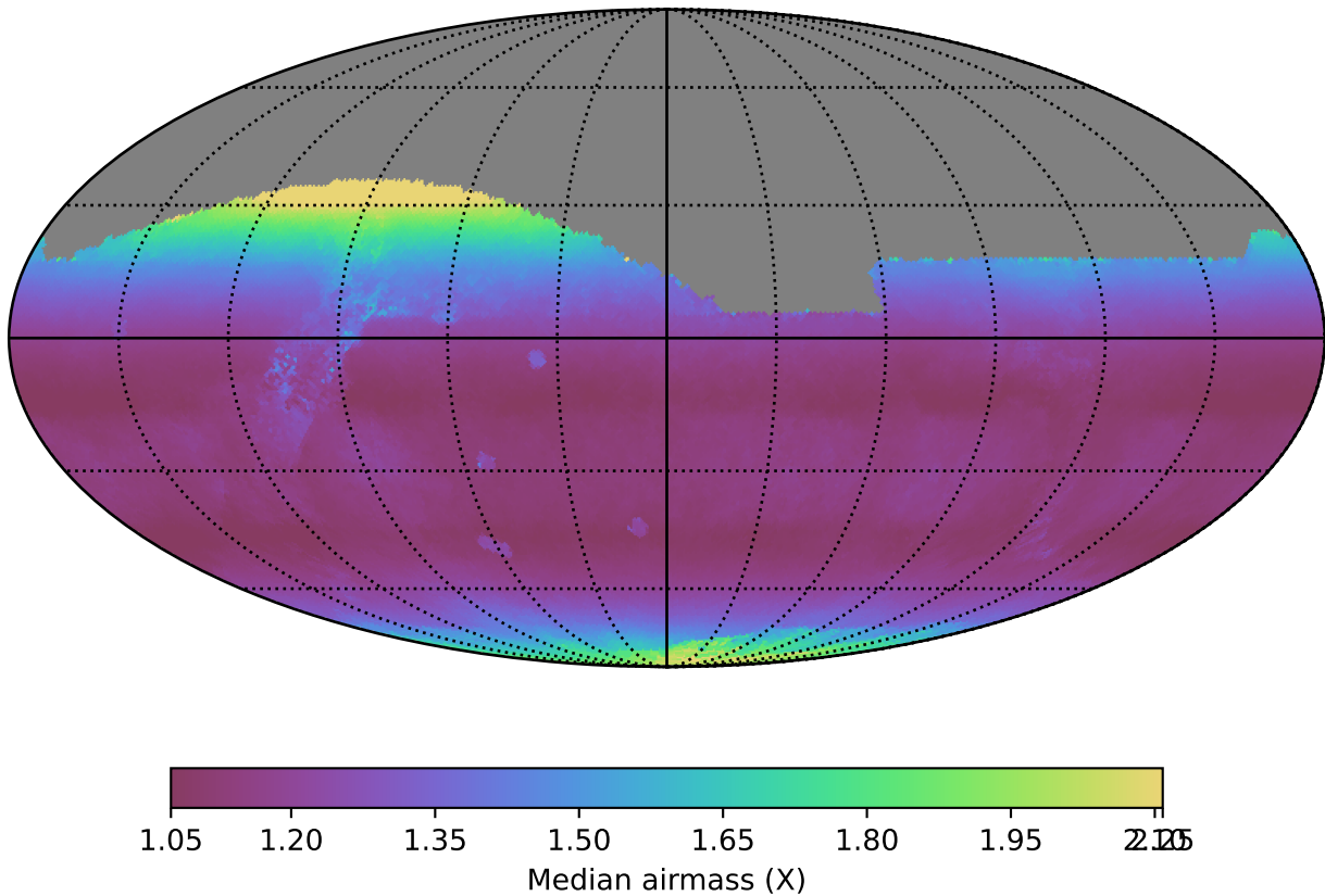
roll_pause_mjdp0_v3.4_10yrs All sky r band: Median airmass
