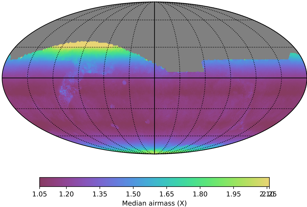
roll_pause_mjdp0_v3.4_10yrs All sky i band: Median airmass
