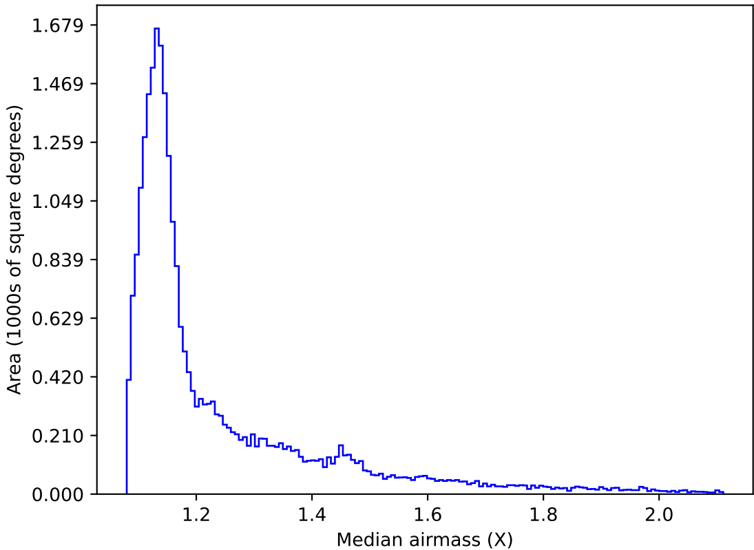
roll_pause_mjdp0_v3.4_10yrs All sky i band: Median airmass
