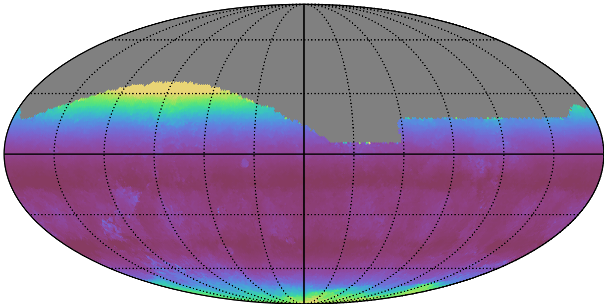
roll_pause_mjdp0_v3.4_10yrs All sky g band: Median airmass
