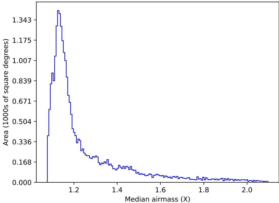
roll_pause_mjdp0_v3.4_10yrs All sky g band: Median airmass
