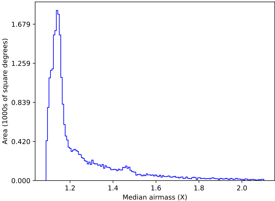
roll_pause_mjdp0_v3.4_10yrs All sky all bands: Median airmass
