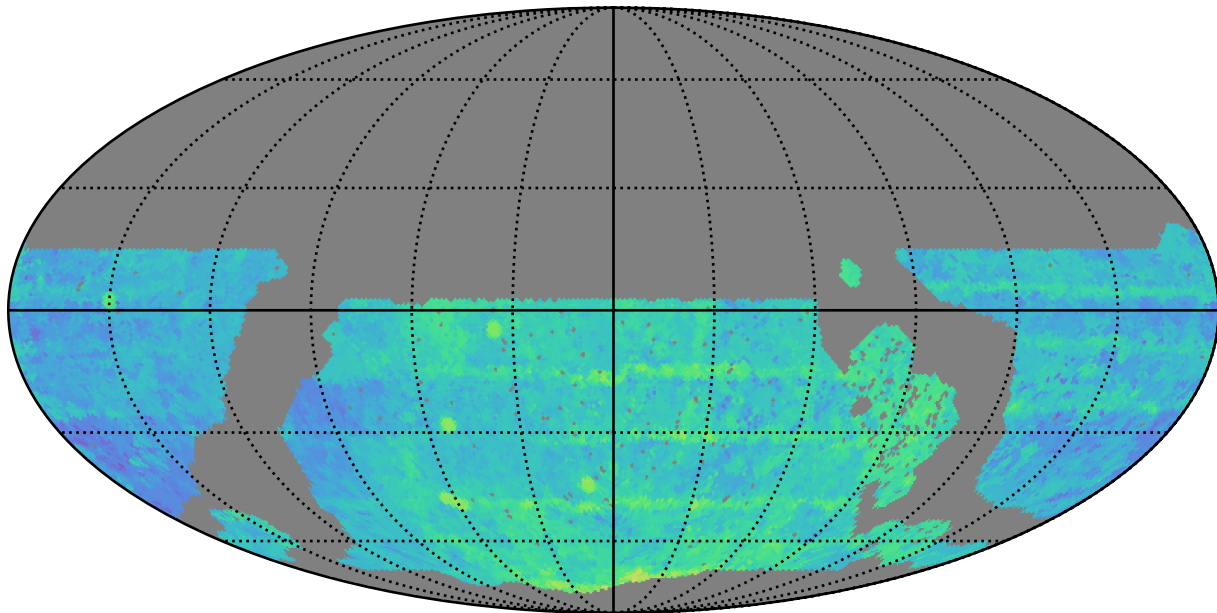
roll_pause_mjdp0_v3.4_10yrs WFD z band: Median Season Length
