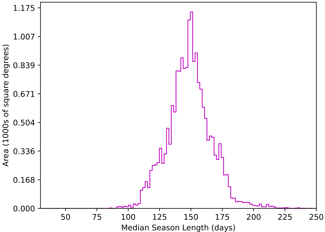
roll_pause_mjdp0_v3.4_10yrs WFD z band: Median Season Length
